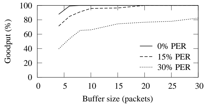
Figure 24. The effect of buffer size to the reliability in TUTWSN using the intermediate buffering scheme algorithm (12 sources, 15 B/s offered load).
