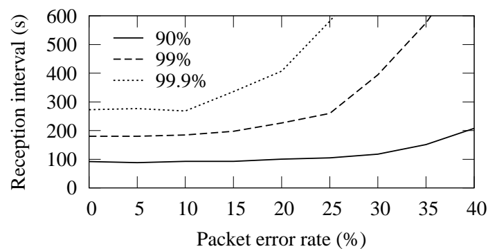
Figure 26. Availability in TUTWSN using the reliable data forwarding (12 sources, 5.5 B/s offered load).
