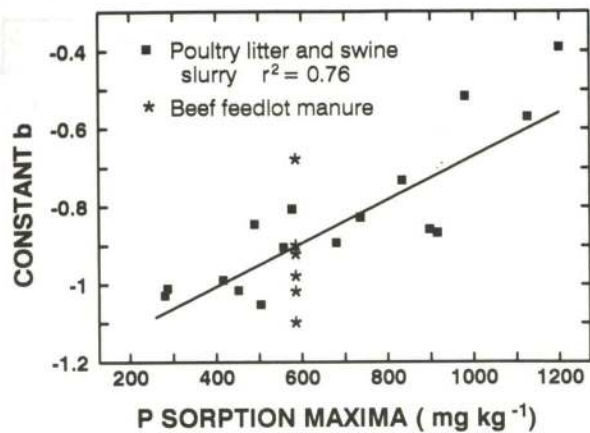
Fig. 2. Relationship between constant b of the strip P successive extraction regression for manured soils and P sorption maximum of corresponding untreated soils.
