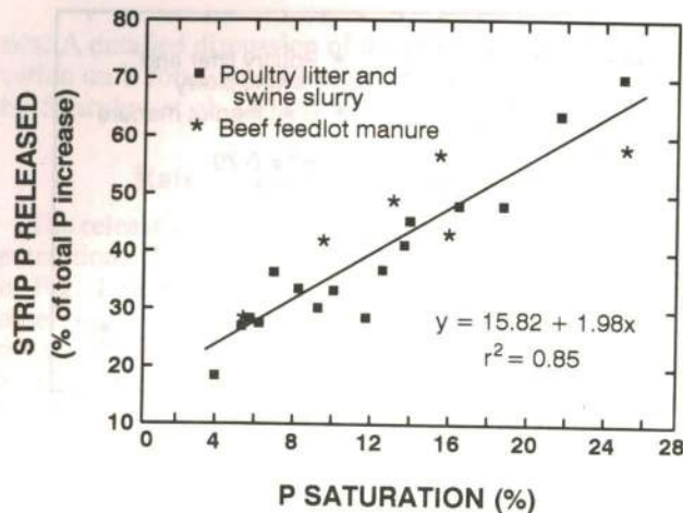
Fig. 4. Relationship between the percentage total P increase with manure application, released as strip P during 15 successive extractions and P sorption saturation.
