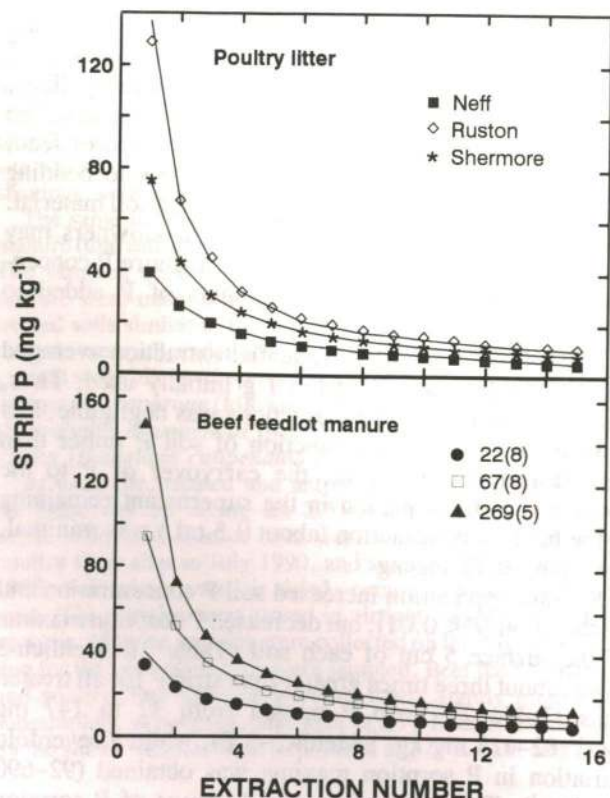
Fig. 1. Strip P released from soils treated with poultry litter and beef feedlot manure during successive extractions.
