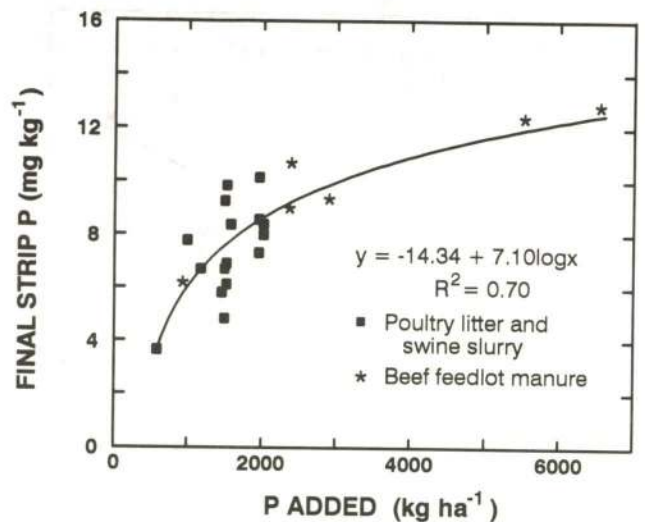
Fig. 5. Relationship between final strip P after 15 successive extractions of treated soils and amount of P added in manure.
