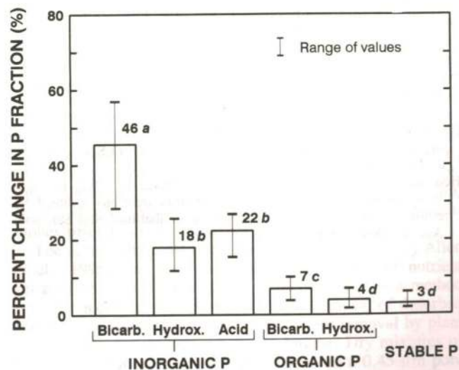
Fig. 6. The decrease in each P fraction as a percentage of strip P released during successive strip extractions of treated soil (number above bar is mean; means followed by different letters are significantly different at P < 0.05 ).
