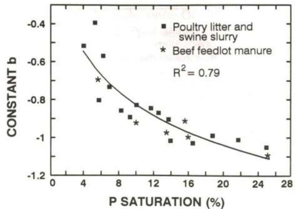
Fig. 3. Relationship between constant b of the strip P successive extraction regression and P sorption saturation of manured soils.
