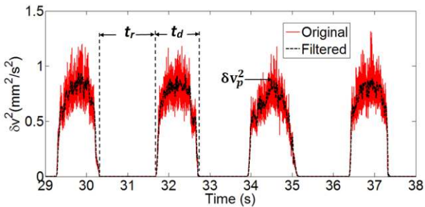
Fig. 5 (Color online) Particle fluctuation velocity, \delta v^2 , over four slump cycles for a drum rotating at a speed of 0.15 RPM. The grey (red online) line represents the raw SVS data whilst the black dash line represents the data after being subject to a Butterworth low pass filter to reduce the noise that originates from the CCD camera.
