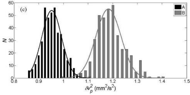
Fig.6 The comparison of the distributions of the following obtained for point A (black) and B (gray) in the drum when rotating at a speed of 0.15 RPM: (a) the rest time, t_r , (b) the avalanche duration time, t_d , and (c) the peak of the particle fluctuation speed of the avalanches, \delta v_p^2 . The data was accumulated from 424 separate avalanches events over 1000 s. The solid curves represent the best fit of a Gaussian distribution to the experimental data, with the averages and standard deviations indicated in Table 1.
