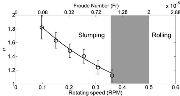
Fig. 10 The variation with drum rotational speed (in the form of Froude number) of the average number of avalanches experienced by particles as they travel from the top to the bottom of the free surface, n , (open circle) as determined from Eq. (7). Gray area represents expected transition region according to previous study of similar systems [1, 3, 36].
