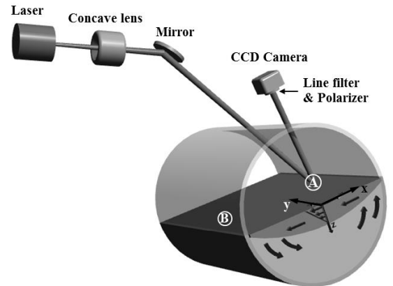
Fig. 2 Schematic of the experimental setup. The points Ⓐ ( x = 50 \text{ mm} , y = 100 \text{ mm} ) and Ⓑ ( x = -50 \text{ mm} , y = 100 \text{ mm} ) were the focus of the SVS analysis reported here.
