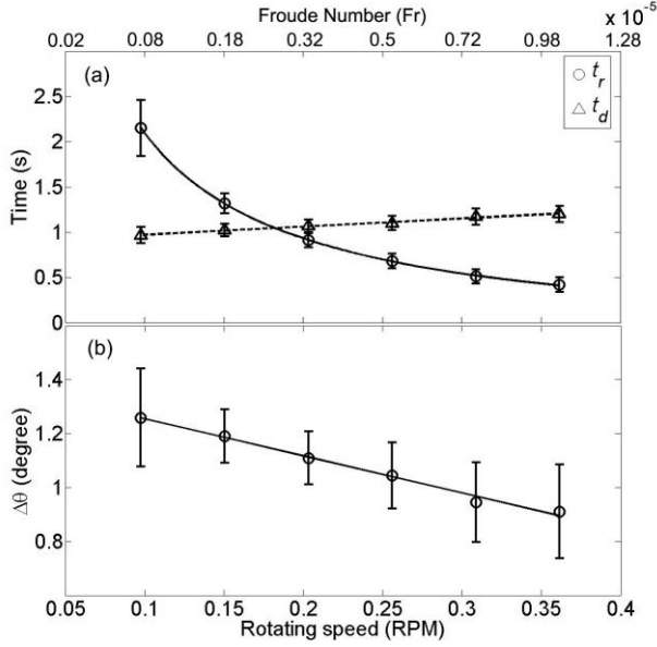
Fig. 9 (a) The comparison of the average rest time, t_r , (open circles) and the average avalanche duration time, t_d , (triangle) vs. drum speed and Froude number, along with the best reciprocal law to t_r (solid line), and line fit to the t_d (dash line) for the point \textcircled{A} . (b) The variation of \Delta\theta with the rotating speeds. Error bars are standard deviations of the distribution of these parameters.
