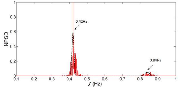
Fig. 8 (Color online) Normalized power spectrum density of the \delta v^2 represented by grey (red online) curve measured in 1000 s, with frequency, f , reduced from 0.1 to 1 Hz. The black dash curve represents the Gaussian fit to the peaks of the data.
