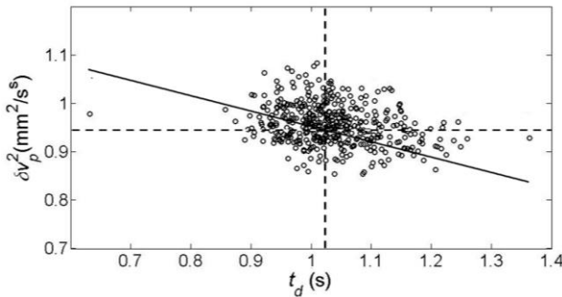
Fig. 7 The peak of the particle fluctuation velocity, \delta v_p^2 , vs. corresponding duration time, t_d , for each of the 424 avalanches observed at point A in the drum when rotating at a speed of 0.15 RPM (open circle) and the fit to this data (solid line). The horizontal and vertical dashed line represents the mean \delta v_p^2 and t_d .
