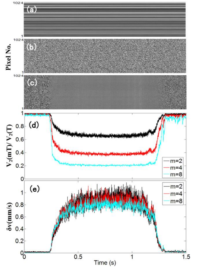
Fig. 4 (colour online) Example SVS results and analysis for glass beads in a drum: (a) intensity across the CCD pixels vs. time when the drum is stationary; (b) intensity across the CCD pixels vs. time when the drum is rotating at a speed of 0.15 RPM and no avalanche event occurs; (c) the same as (b) except an avalanche event has occurred in the period of around 0.25-1.25 s; (d) intensity variance ratio, Eq. (1), evaluated from the data in (c); and (e) root-mean-particle fluctuation velocity ( \delta v ) obtained from variance ratio.
