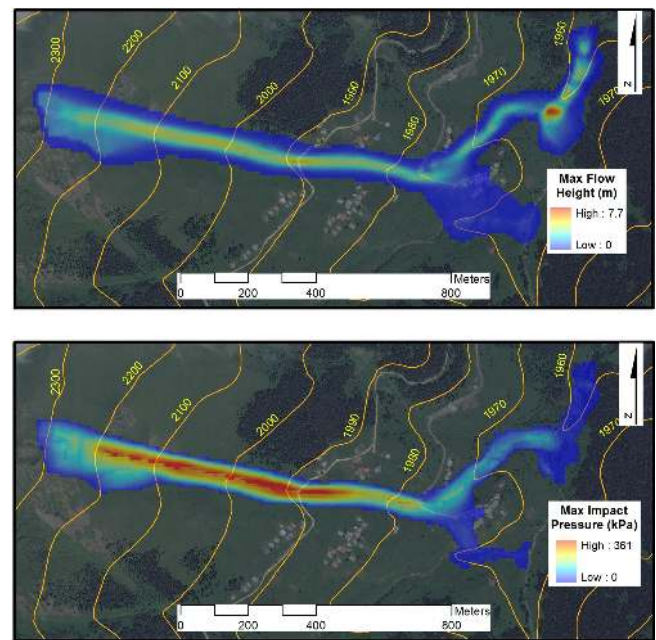
Fig. 11. Simulation result of Yaylaönü project area: maximum flow height (top) and maximum impact pressure (bottom).
