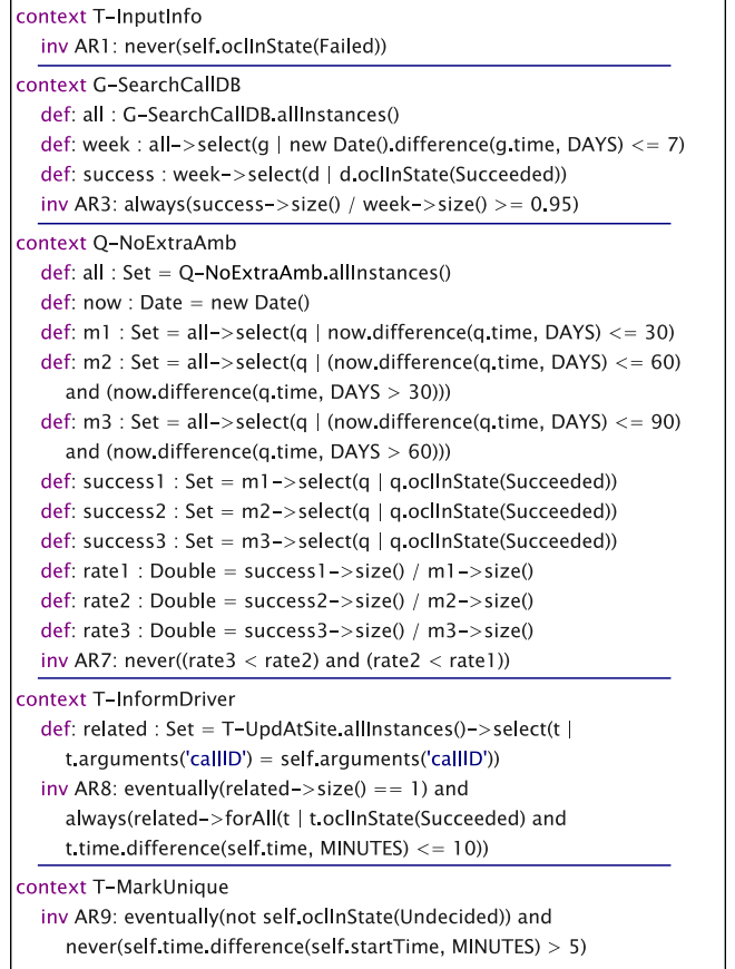
Figure 7: Some AwReqs formalized in OCL_{TM} .
