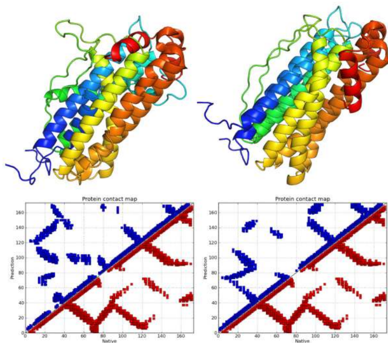
Figure 6. Structural alignments and comparative contact maps of the maximum Q score structures for 2FHA, with the “homologs excluded” prediction on the left ( Q = 0.319 , RMSD 12.383\text{\AA} ) and the “homologs allowed” prediction on the right ( Q = 0.476 , RMSD 8.781\text{\AA} ).
