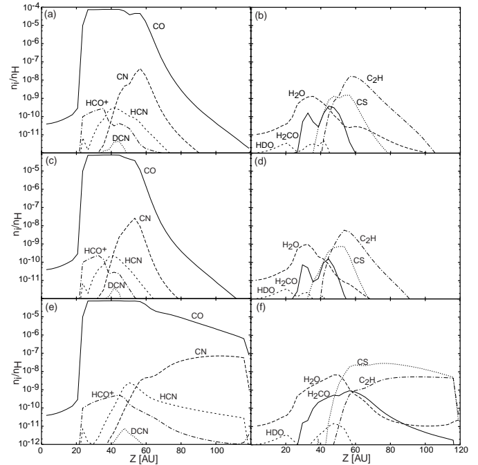
Fig. 7. Vertical distribution of molecules at R = 105 AU and t = 1 \times 10^6 yr. Panels a) and b) are for Spectrum A, panels c) and d) are for Spectrum B and panels e) and f) for Spectrum C.
