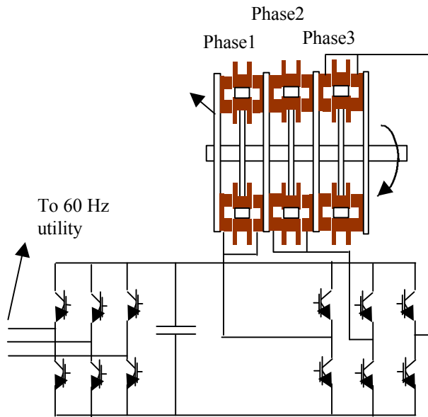
Figure 3. Expansion for multimodule generation.
