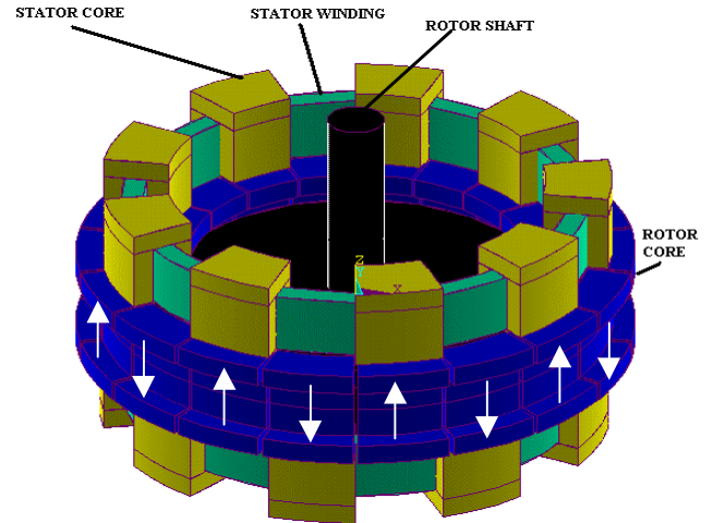
Figure 2. PM Generator with Toroidal Winding
