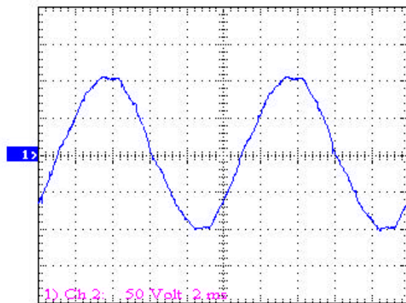
Figure 6. Open circuit voltage
