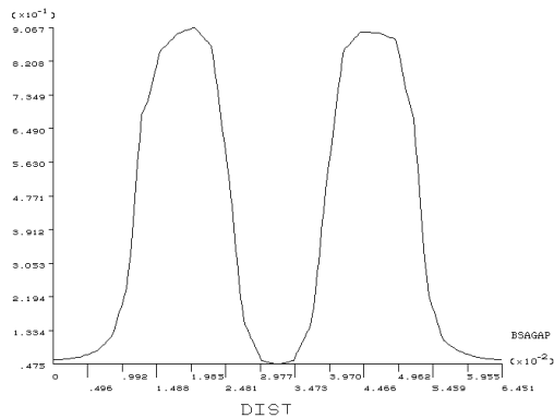
Figure 5. Flux density at no-load condition
