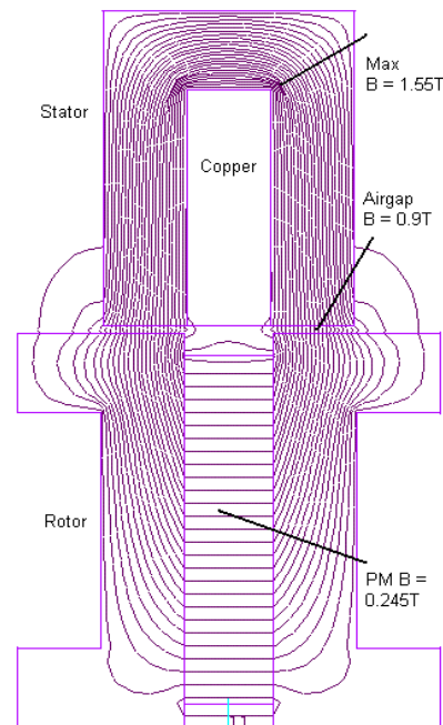
Figure 4. Flux density at no-load condition
