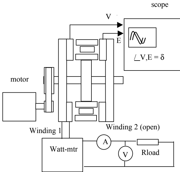
Figure 8. Experimental set-up
