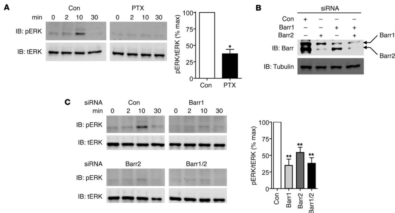
Figure 4 Nicotinic acid–stimulated phosphorylation of ERK. (A) GPR109A-expressing HEK-293 cells were stimulated with 200 \mu M nicotinic acid, and cell lysates were analyzed for phosphorylated ERK (pERK) at varying times. Agonist stimulated activation of ERK in the presence or absence of pertussis toxin. tERK, total ERK. * P = 0.027 versus control. (B) Expression of \beta -arrestin decreased after siRNA treatment. (C) Agonist stimulated ERK activation in the presence of control, \beta -arrestin1, \beta -arrestin2, or \beta -arrestin1 and \beta -arrestin2 siRNA. Graph shows phosphorylation of ERK 10 minutes after stimulation. ** P < 0.05 versus control. Data are mean \pm SEM of 3–6 independent experiments.
