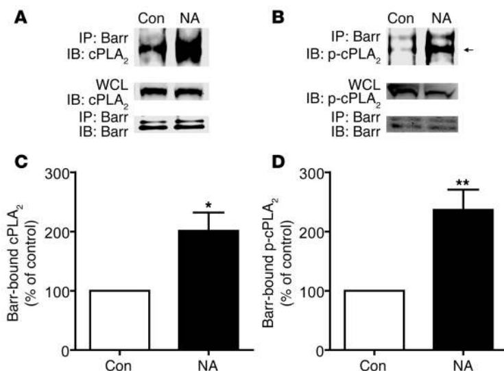
Figure 5 Nicotinic acid–induced binding of \beta -arrestin to cPLA 2 and phosphorylated cPLA 2 . (A and B) GPR109A-expressing HEK-293 cells were stimulated with 10 \mu M nicotinic acid or control for 10 minutes. Nicotinic acid stimulation increased binding of \beta -arrestin to cPLA 2 (A) and phosphorylated cPLA 2 (p-cPLA 2 ) (B) . Arrow indicates phosphorylated cPLA 2 band. Equivalent amounts of cPLA 2 were present in each whole cell lysate (WCL). Equal amounts of \beta -arrestin were immunoprecipitated in control and nicotinic acid–treated samples. Moreover, \beta -arrestin was not immunoprecipitated with preimmune serum (not shown). (C and D) Binding of \beta -arrestin to cPLA 2 (C) and phosphorylated cPLA 2 (D) . * P = 0.0075 , ** P = 0.015 versus control. Data are mean \pm SEM of 5 independent experiments.
