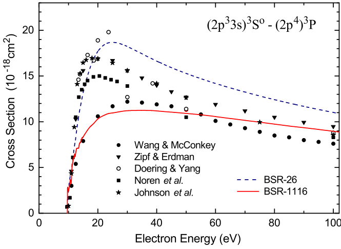
FIG. 15. (Color online) The (2p^3 3s)^3 S^o - (2p^4)^3 P emission cross sections as a function of electron energy. The present BSR-1116 results are compared with those from a BSR-26 model [8] and experimental data of Wang and McConkey [49], Zipf and Erdman [48], Doering and Yang [39], Noren et al. [50], and Johnson et al. [47].
