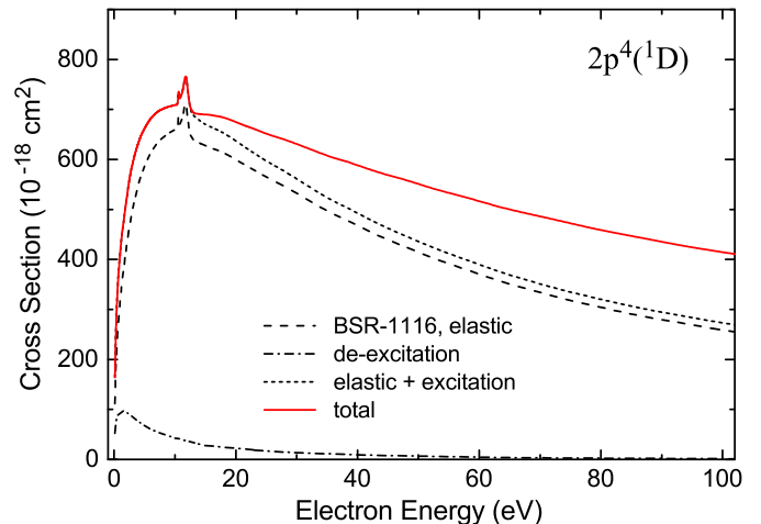
FIG. 23. (Color online) Angle-integrated elastic, elastic + excitation, elastic + excitation + ionization, and grand total cross sections for electron collisions with oxygen atoms in their (2p^4)^1D metastable state. In this case, the grand total cross sections also contain deexcitation through superelastic scattering.
