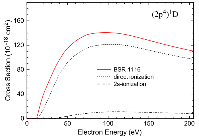
FIG. 20. (Color online) Angle-integrated cross sections for electron impact ionization of oxygen atoms in the metastable state (2p^4)^1D . The direct ionization cross sections and the partial contribution of the 2s -ionization are also shown.
