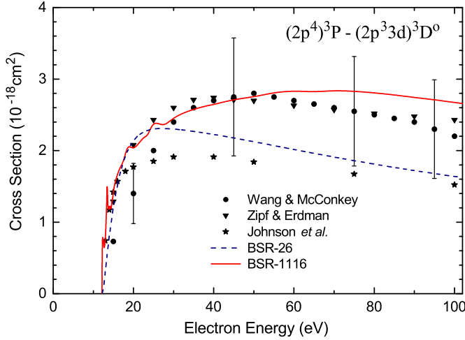
FIG. 16. (Color online) The (2p^4)^3 P - (2p^3 3d)^3 D^o emission cross sections as a function of electron energy. The present BSR-1116 results are compared with those from a BSR-26 model [8] and experimental data of Zipf and Erdman [48], Wang and McConkey [49], and Johnson et al. [47].
