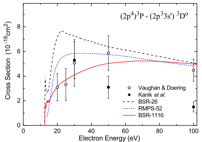
FIG. 8. (Color online) The excitation cross sections for the allowed (2p^4)^3P - (2p^3 3s')^3D^o transition. The present BSR-1116 results are compared with those from a BSR-26 model [8], a 52-state RMPS calculations (RMPS-52) [11], and experimental data of Vaughan and Doering [37] and Kanik et al. [40].
