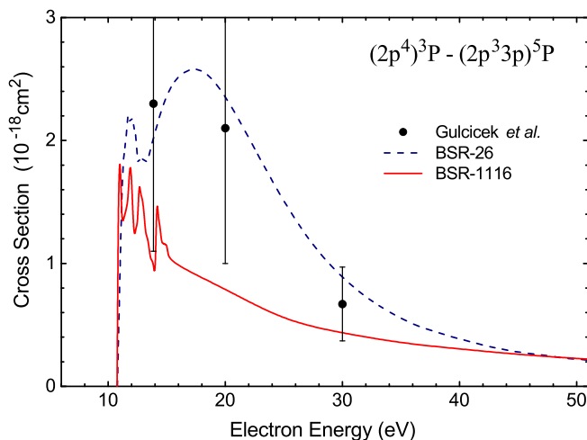
FIG. 14. (Color online) The excitation cross sections for the (2p^4)^3P - (2p^3 3p)^5P transition as a function of electron energy. The present BSR-1116 results are compared with those from a BSR-26 model [8] and experimental data of Gulcicek et al. [45].
