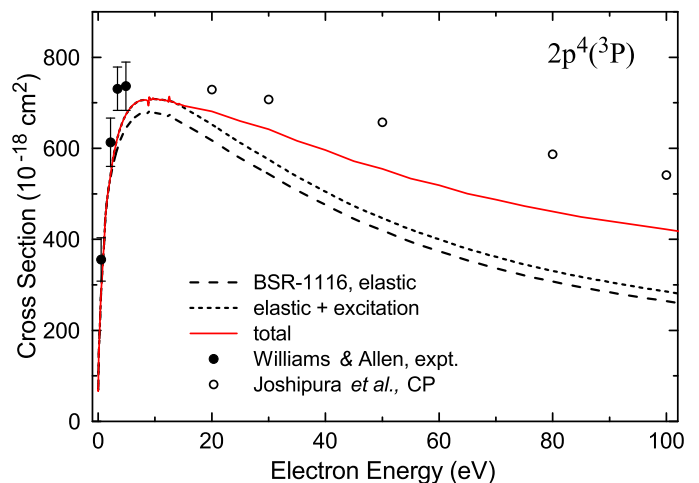
FIG. 22. (Color online) Angle-integrated elastic, elastic + excitation, and grand total (elastic + excitation + ionization) cross sections for electron collisions with oxygen atoms in their (2p^4)^3P ground state. The experimental results of Williams and Allen [29] and theoretical data of Joshupura et al. obtained from complex potential (CP) method [54] have also been shown.
