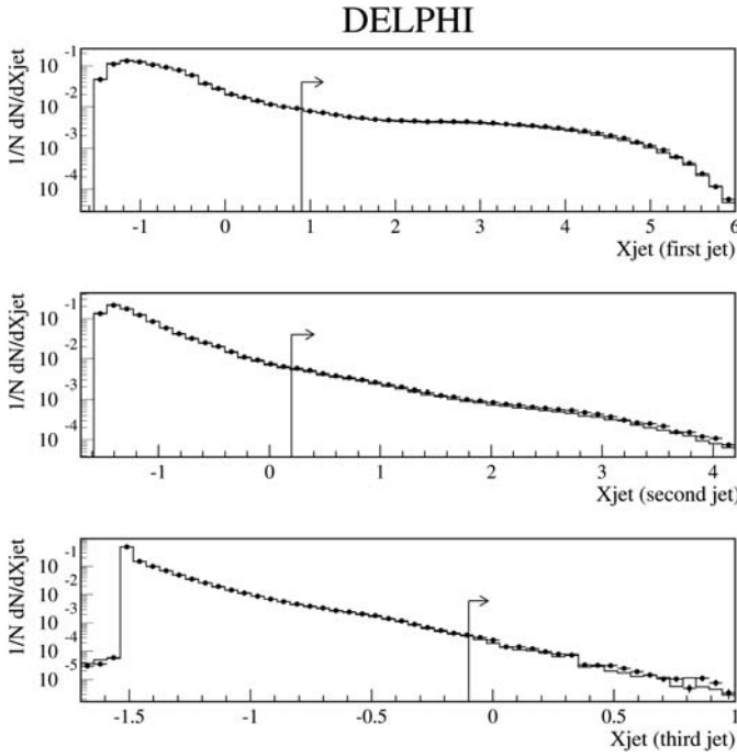
Fig. 23. Distribution of the b -tagging variables for the first three jets, ordered according to their b -tagging variable, for Z data (dots) and simulation (histogram). The arrows show the positions of the cuts used to select the b jets. The figure is from [22]
