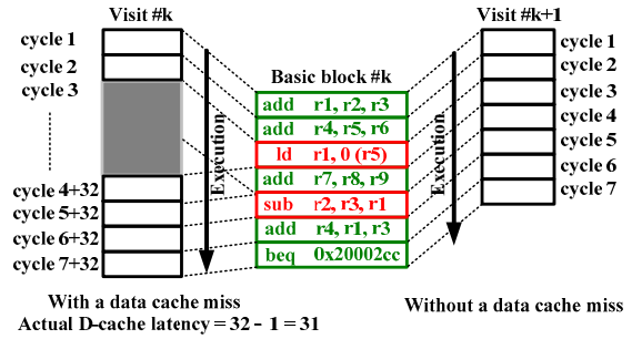
Figure 3. Example of Off-chip CPI Calculation w/ and w/o a Data Cache Miss in a Basic Block
