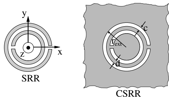
FIG. 1. Geometries of the SRR and the CSRR.
