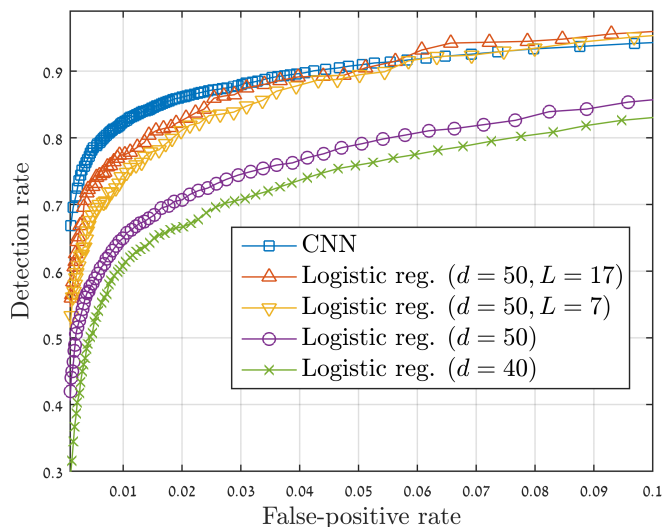
Fig. 7: ROC curves for the logistic regression and the CNN classifiers.
