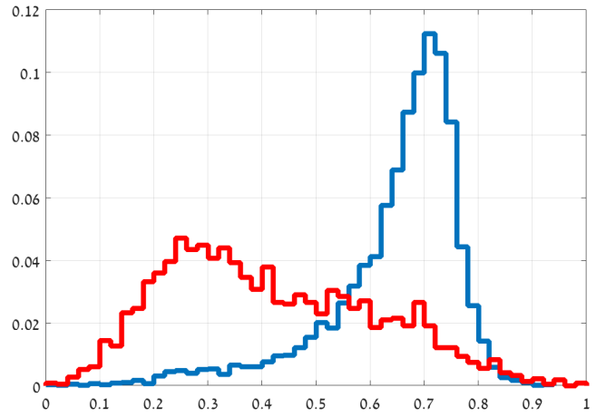
Fig. 2: A histogram of the 5th MFC coefficient. Red: cry events, blue: other events.
