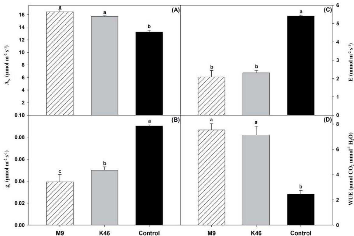
Figure 4. A) CO 2 Assimilation rate (A N ), B) stomatal conductance (g s ), C) transpiration (E), and D) water use efficiency (WUE) of Habanero pepper plants inoculated with Bacillus spp. (M9 and K46) and not inoculated (control).
