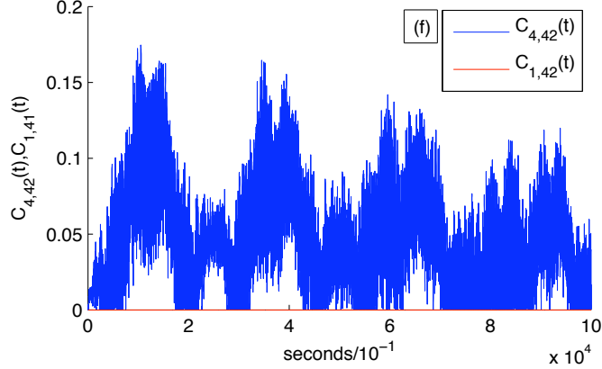
FIG. 3: Entanglement dynamics in the model. Here we plot the concurrence between the number of particles n_4 at the node 4 and the insisting edge 24 (blue line). We see a non trivial evolution which shows equilibration at large times. Red line shows the same quantity for the node 1, showing that an edge only entangles with the nodes it comes from and therefore C_{1,42} = 0 during the whole evolution.
