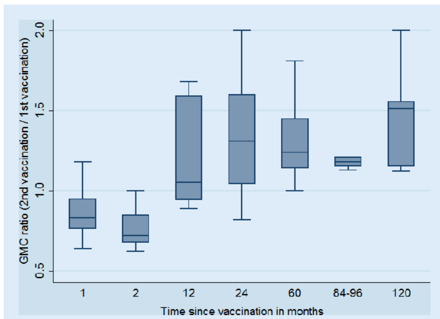
Fig. 8 ▲ Ratios of immunoglobulin G (IgG) concentration
