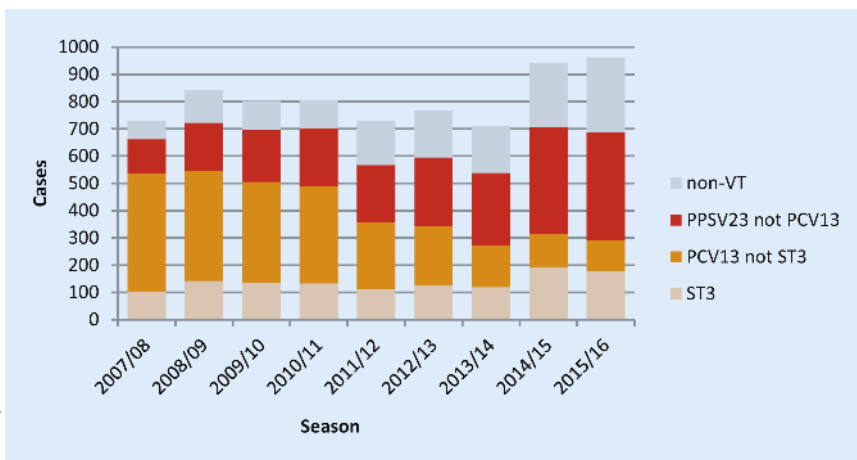
Fig. 3 ▲ Serotype distribution of the IPD cases recorded on PneumoWeb in seniors 60 years and over, absolute case numbers ST3 = serotype 3, non-VT = serotypes not contained in any vaccine Seasonal variations of case numbers may reflect real differences in incidence, but may also result from surveillance artefacts, e.g. changing numbers of laboratories participating in PneumoWeb
