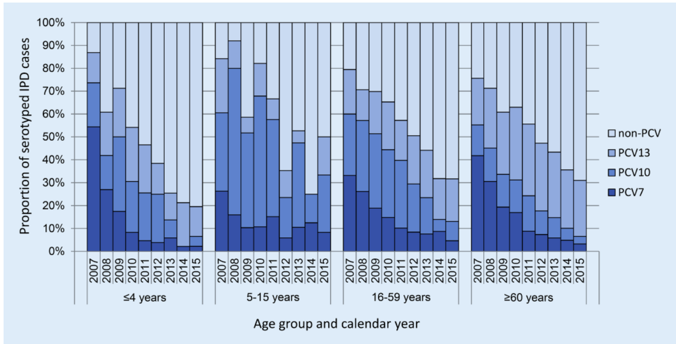
Fig. 2 ▲ Relative distribution of serotypes contained in the different pneumococcal conjugate vaccines of the IPD cases recorded in PneumoWeb, by age group and year of disease
