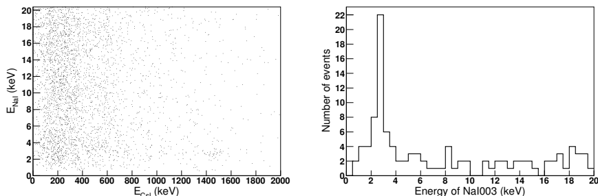
Figure 2. (left) A scatterplot of NaI-003 signals (vertical) versus CsL crystal energies (horizontal) for coincidence events. (right) The NaI-003 crystal’s energy distribution for events in coincidence with a 1460 \pm 150 keV \gamma -ray in one of the CsI crystals. The ^{40}\text{K} events correspond to the distinct peak near 3 keV in the NaI-003 detector’s energy spectrum.
