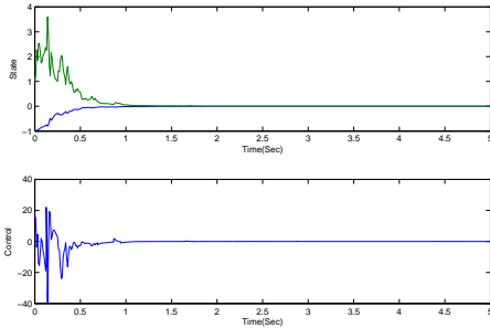
Fig.1. The responses of closed-loop system with Markovian switching.
