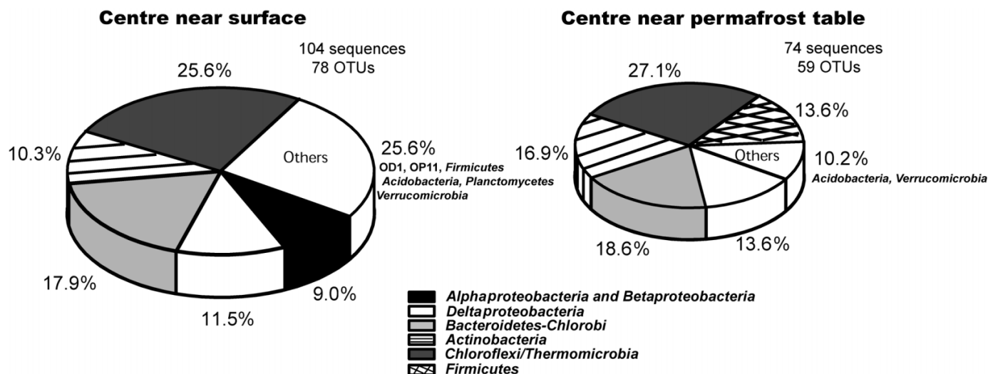
Fig. 1. Relative abundance and affiliation of bacterial operational taxonomic units (OTUs) in a low-centred polygon on Samoylov Island, Lena Delta, northeastern Siberia.
