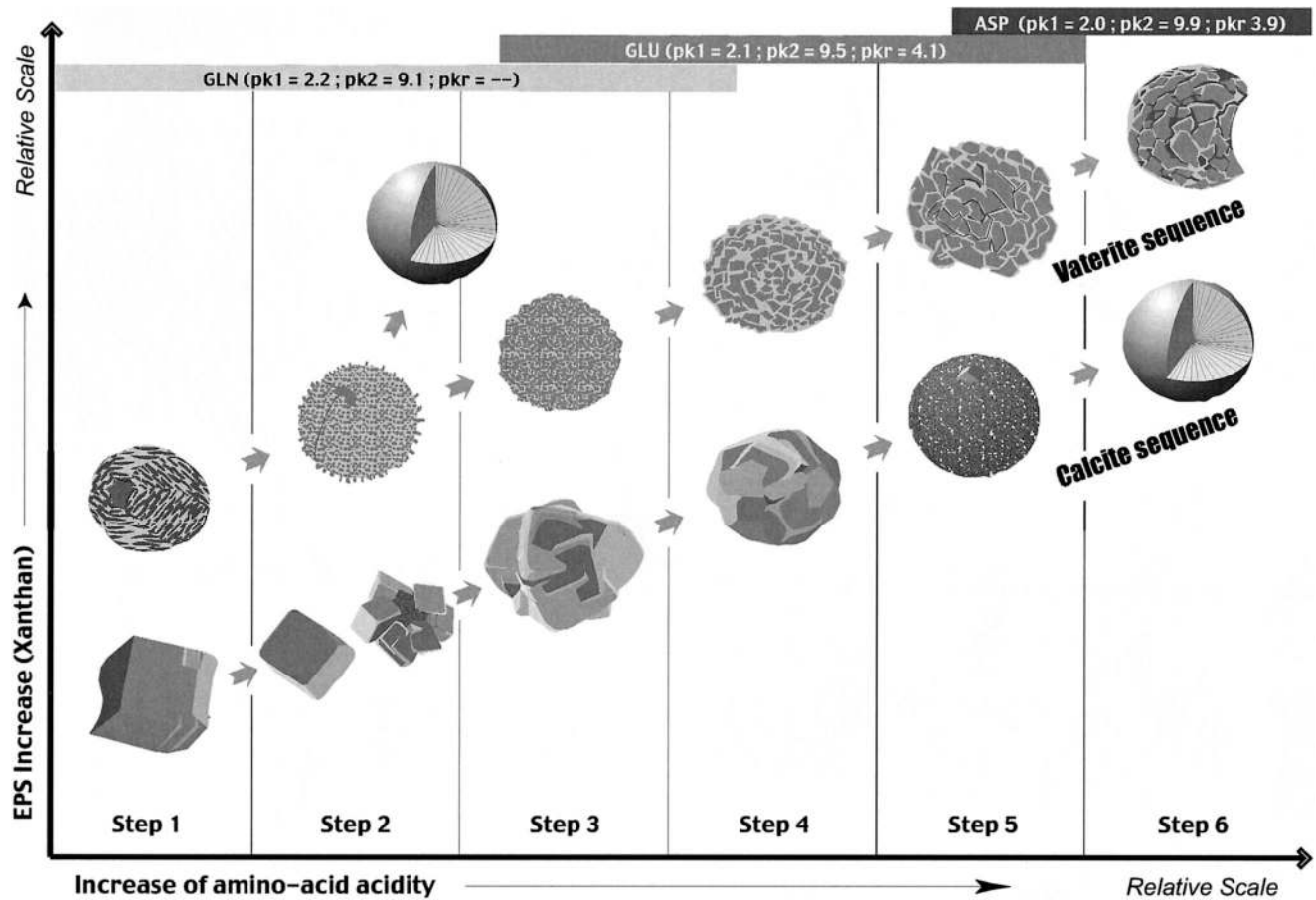
Fig. 5.—Sequences of calcite and vaterite morphologies obtained during the abiotic experiment. This sketch shows the morphologies related to increasing amino acid acidity and xanthan content. Scales are relative. The various domains of influence of amino acids are shown. Six main steps can be described for both vaterite and calcite. The calcite sequence starts with rhombohedra. Size of monocrystals forming the clusters decreases from Step 1 to Step 6 until they form needles. The general shape of calcite evolves from rhombohedra to fibro-radial spherulites. Vaterite sequence: vaterite is always precipitated as spheres. The monocrystals constituting the spheres increase in size from Step 1 (short needles) to Step 6 (large hexagons). Between Step 2 and Step 3, vaterite can occur as fibro-radial spherulites. Sketches were traced from photographs.
