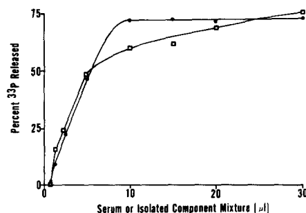
FIG. 4. Dose-dependent lysis of E. coli K12 W1485 by the 11 isolated proteins of the cytolytic alternative pathway and lysozyme. Incubations at 37°C for 60 min were performed as described in Methods using the isolated component mixture or C4-depleted serum. Lysozyme concentrations used were 10 μg egg white lysozyme/ml isolated component mixture. ●, isolated component mixture plus lysozyme; □, C4-depleted serum.
