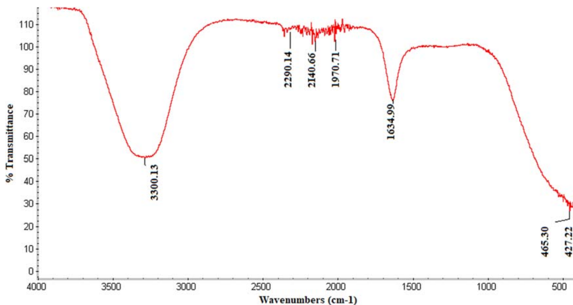
Figure 2: IR spectra of the biosynthesized AgNPs prepared with aqueous R. officinalis leaf extract.
