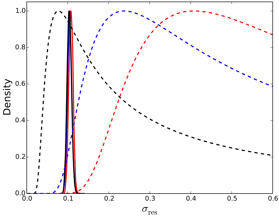
Fig. 3.— Robustness of the posterior distribution for \sigma_{\text{res}} (solid lines) with respect to three different prior specifications (dashed lines) Black: \sigma_{\text{res}}^2 \sim \text{INV}\text{GAMMA}(0.003, 0.003) ; blue: \sigma_{\text{res}}^2 \sim \text{INV}\text{GAMMA}(0.03, 0.03) ; red: \sigma_{\text{res}}^2 \sim \text{INV}\text{GAMMA}(0.1, 0.1) . Since the three posterior distributions are very similar, we conclude that the posterior distribution of \sigma_{\text{res}} is largely insensitive to its prior specification (assuming \Lambda\text{CDM} ). Densities have been normalized to their peak for ease of comparison. In the rest of this paper, we use \sigma_{\text{res}}^2 \sim \text{INV}\text{GAMMA}(0.003, 0.003) .
