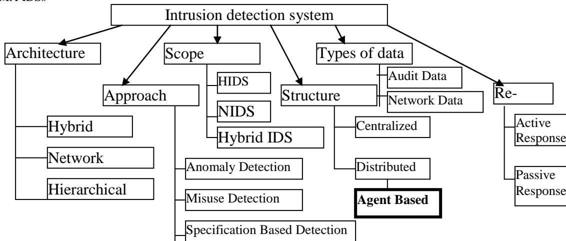
Figure 1: Taxonomy of Intrusion Detection System
