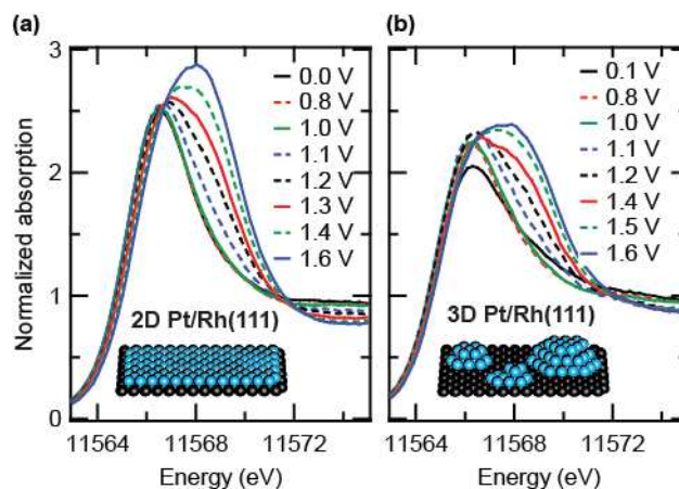
Figure 2. In situ Pt L_3 HERFD XAS for 1 ML Pt/Rh(111) in 0.01 M HClO_4 : (a) 2D Pt film, (b) 3D Pt islands. Spectra were recorded in the order of increasing electrochemical potentials.
