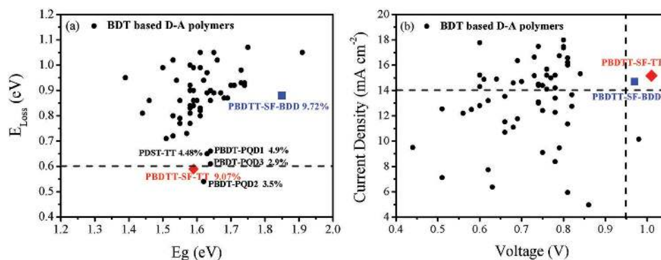
Figure 1. a) Correlation between energy loss and band gap for PBDT-TT-SF-TT, PBDT-TT-SF-BDD, and BDT and/or TT-based D–A polymers from literature. b) J_{sc} and V_{oc} for PBDT-TT-SF-TT, PBDT-TT-SF-BDD, and BDT and/or TT-based D–A polymers from literature. Black spots: literature reported BDT and/or TT-based D–A polymers, red diamond and blue square: PBDT-TT-SF-TT and PBDT-TT-SF-BDD.
