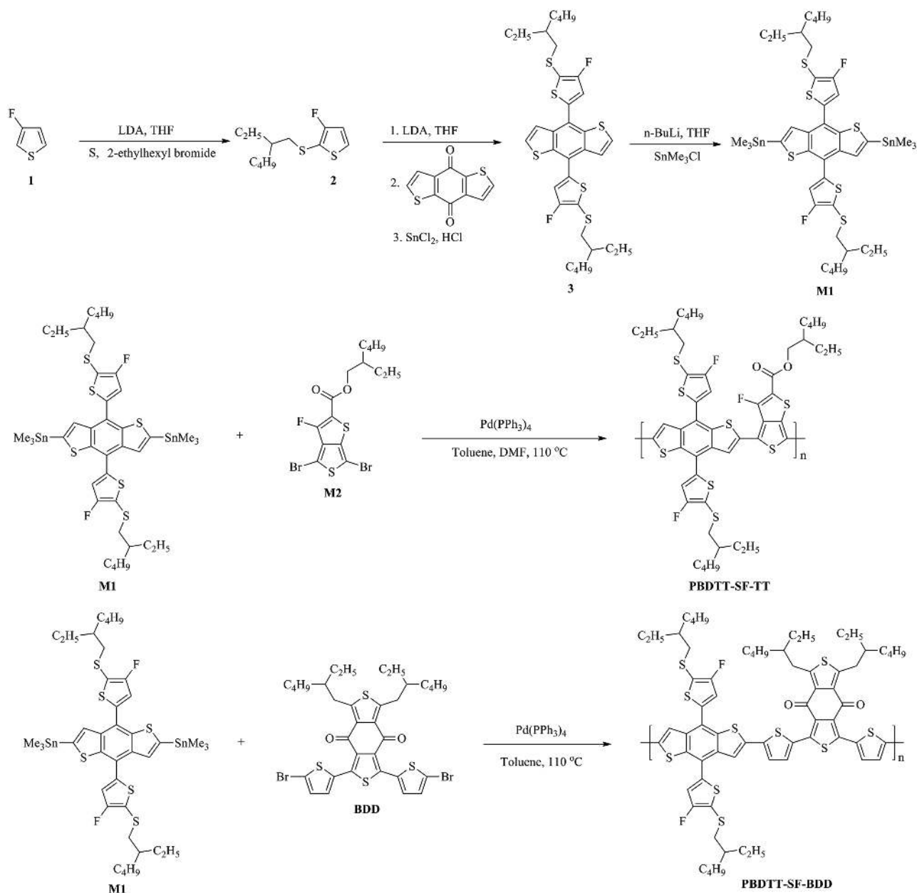
Scheme 1. Chemical structures and synthetic routes of monomer M1 (bis-stannylated-(fluorinated-alkylthiophenyl)-BDT), namely, BDTT-SF and the target polymer PBDTT-SF-TT and PBDTT-SF-BDD.
