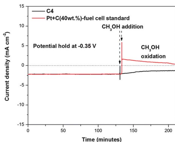
Fig. 10 Chronoamperometric responses of C_4 and Pt/C at -0.35 \text{ V} in O_2 saturated 0.1 M KOH without and with methanol at a rotating rate of 1600 rpm.
