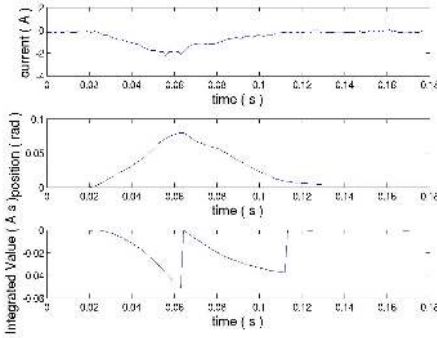
Fig. 12. Receiving soft ball
