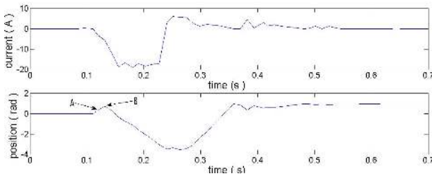
Fig. 3. kick with current detection system
