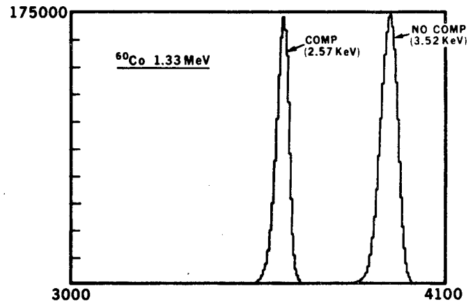
Fig. 8: ^{60}\text{Co} 1.33 MeV line shapes (compensated and uncorrected) for the p-type detector C used at only 1200 V with a peaking time of 3 \mu s.
