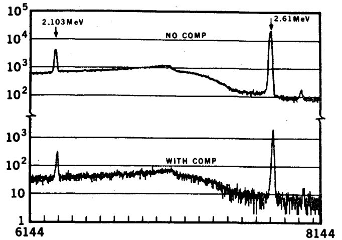
Fig. 12 As Fig. 10, but the energy range is approximately from 2.1 MeV to 2.7 MeV.
