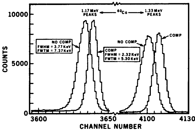
Fig. 6: As Fig. 5 but a peaking time of 2 \mu s was used. Note the slight tailing on the high energy side of the peak due to a slight excess of correction being used in this case.
