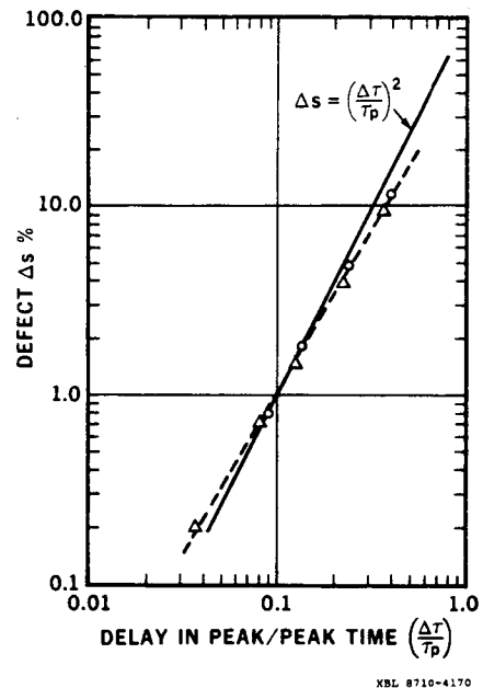
Fig. 2: The dotted line shows the relationship between the output signal ballistic deficit and the peak delay; these results are derived from Fig. 1. The circles are points for the 6th order Gaussian while the triangles are points for the quasi-triangular. The full line shows a square law relationship.
