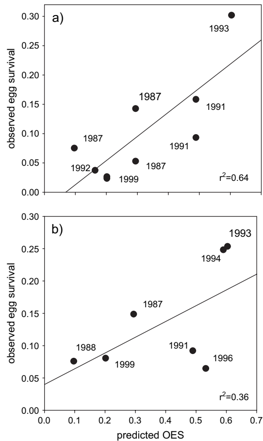
Figure 6. Observed egg survival from ichthyoplankton surveys (proportion surviving to stage III) from following cohort development (a) and from seasonal stage-specific egg production curves (b) vs. predicted oxygen-related egg survival (OES).
