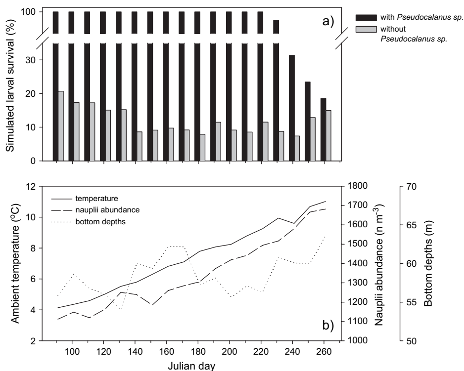
Figure 8. Seasonal variability in simulated larval survival (averaged 1986–1999) in SD 25 from a2 coupled hydro-/trophodynamic model based on an idealized prey field, with and without Pseudocalanus sp. (a), and average ambient environmental variables encountered by surviving larvae (runs without Pseudocalanus sp.), i.e. nauplii abundance, temperature, and bottom depth after drift period as a measure of transport (b), modified after Hinrichsen et al. (2002b).
