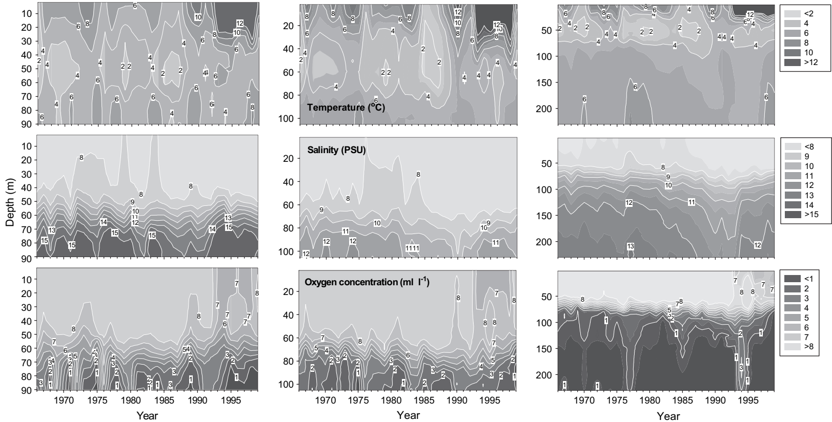
Figure 2. Temperature, salinity, and oxygen concentrations during the main spawning season (second quarter 1966–1989, third quarter 1990–1999) in the Bornholm Basin (left), the Gdańsk Deep (middle), and the Gotland Basin (right).
