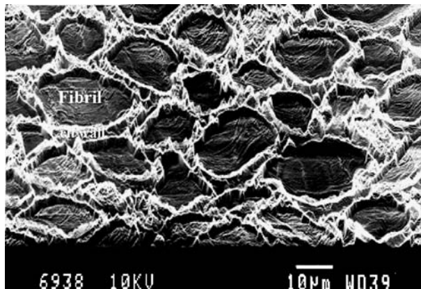
Figure 7 Topographical SEM micrograph shows the fibrils (sclerenchyma cells) and the wall thickness between the fibrils.
