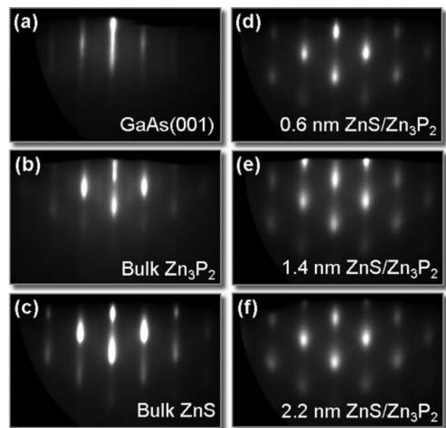
FIG. 1. In situ RHEED images of an (a) atomic hydrogen treated GaAs(001) surface, (b) 150 nm bulk Zn 3 P 2 film, (c) 150 nm bulk ZnS film, (d) 0.6 nm ZnS/Zn 3 P 2 , (e) 1.4 nm ZnS/Zn 3 P 2 , and (f) 2.2 nm ZnS/Zn 3 P 2 . All RHEED images were obtained using a 20 keV electron beam incident along the [011] direction of the GaAs(001) surface.
