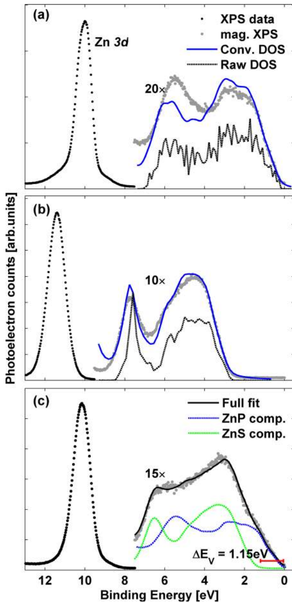
FIG. 3. XPS data of the valence-band region for (a) bulk \text{Zn}_3\text{P}_2 , (b) bulk \text{ZnS} , and (c) a 1 nm \text{ZnS}/\text{Zn}_3\text{P}_2 heterojunction interface. For bulk samples, the raw and convoluted VB-DOS calculations that were used for determining the VBM are displayed. For the interface sample, the valence-band region was fit using a superposition of the bulk \text{ZnS} and bulk \text{Zn}_3\text{P}_2 valence-band spectra.
