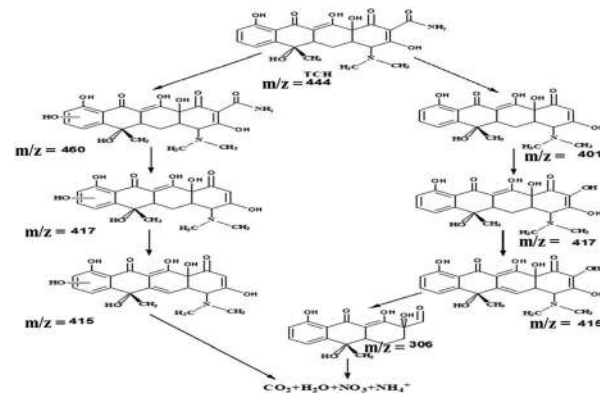
Scheme 2 The degradation pathway via different intermediates.
