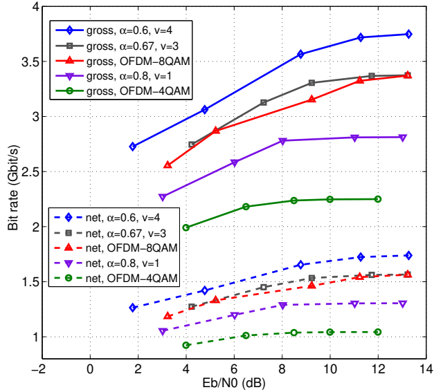
Figure 9. Gross and net bit rates of SEFDM signals at 60 GHz mm-wave through 3 meters wireless and 250 meters MMF fiber transmission with 4QAM symbols.
