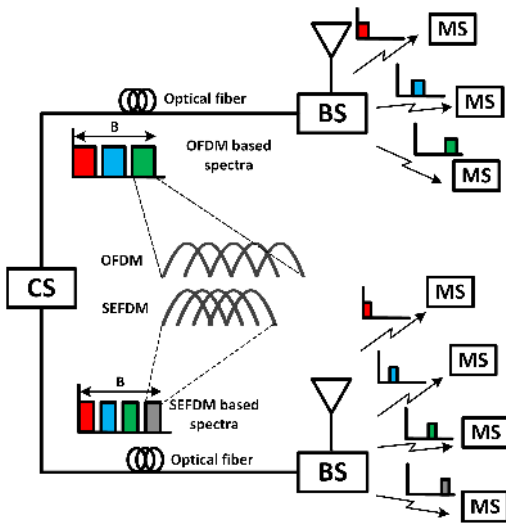
Figure 1. Application scenario of SEFDM in fiber wireless networks where CS indicates central station, BS indicates base station and MS indicates mobile station. Both OFDM and SEFDM sub-carrier packing schemes for each band are illustrated.
