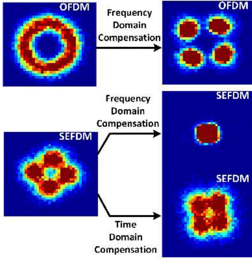
Figure 6. Constellation diagrams for OFDM and SEFDM (i.e. \alpha=0.8 ) signals before and after channel compensation.
