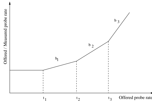
Figure 7.1: Plot of offered prob rate / measured probe rate as a function of the offered probe rate. The three segments b_1 - b_3 corresponds to three congested links while t_1 - t_3 are breakpoints between congested links.
