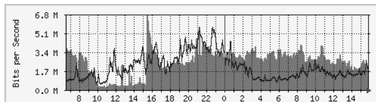
Figure 1.5: MRTG day trace. 5 minute intervals.
