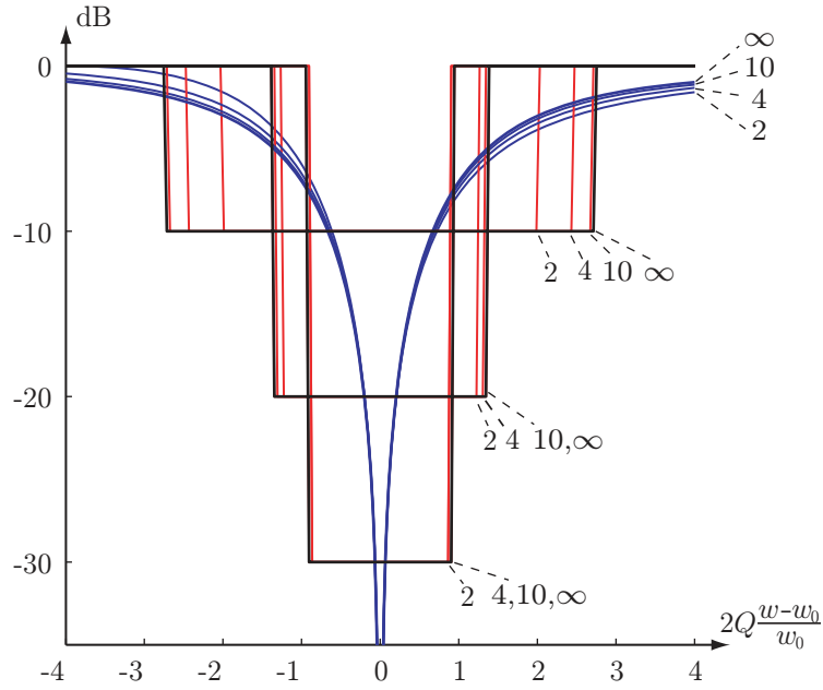
Figure 4: Reflection coefficient of a resonance circuit for different Q factors and Bode-Fano matching networks. The Q factors Q = 2, 4, 10, \infty and the Bode-Fano limits corresponding to -10, -20, -30 dB are shown.
