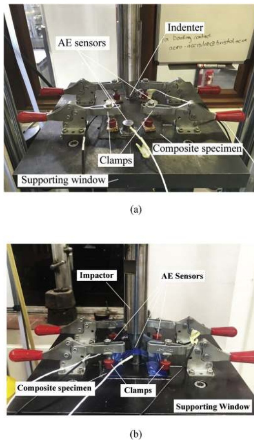
Fig. 1. a) Quasi-static indentation, and b) LVI test setups.
