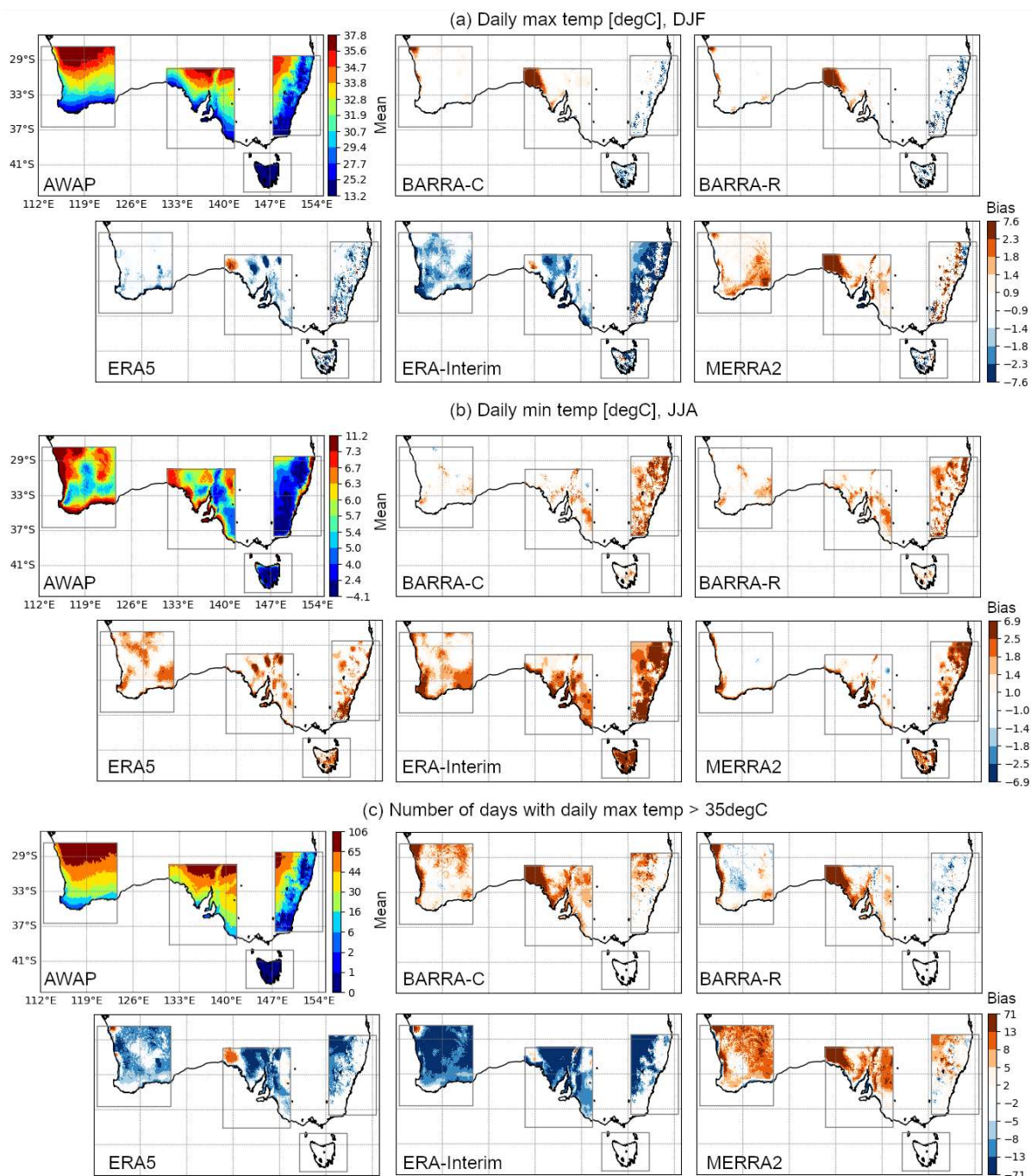
730 Figure 3: Mean difference in (a) summer (DJF) daily maximum temperature, (b) winter (JJA) daily minimum temperature and (c) number of days with temperature exceeding 35 °C, in various models during 1990-2018, with respect to AWAP. The models are regridded onto the AWAP grid with the nearest-neighbour interpolation.
