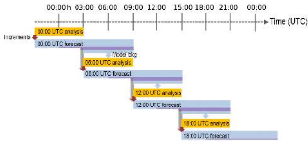
Figure 2. Cycling set-up of BARRA-R at base time t_0 = 00:00 , 06:00, 12:00, and 18:00 UTC. Each UM forecast is initialized at t_0 - 3 h by the previous forecast (grey arrows) with increments from the current analysis (red arrows). The purple bars indicate the time steps of the model states that have been archived.
