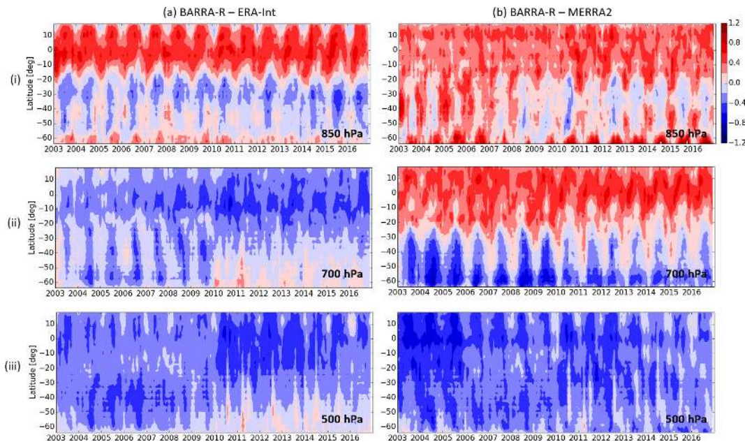
Figure 8. Hovmöller plots of the monthly difference in zonal mean air temperature (K) at 00:00 UTC and three pressure levels, (row i) 850, (ii) 700, and (iii) 500 hPa, between (a) BARRA-R and ERA-Interim and between (b) BARRA-R and MERRA-2.
