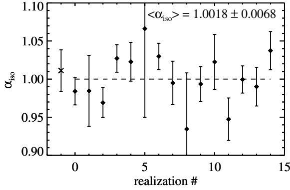
Fig. 17. Measurements of \alpha_{\text{iso}} ( =\alpha_t = \alpha_r ) for the 15 sets of mock spectra and for the data (realization = -1). The large errors for realization 5 and 8 are due to the very low significance of the BAO peak found on these two sets.
