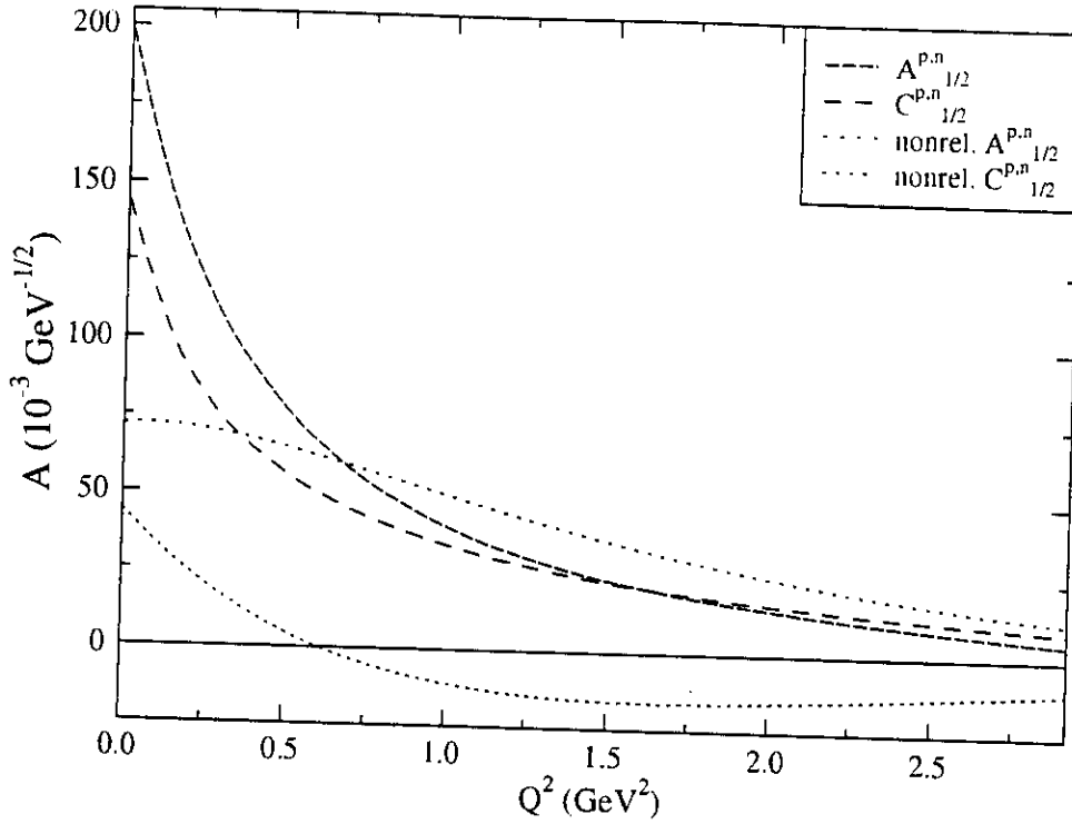
Figure 10: \Delta(1620) electroexcitation helicity amplitudes. Key as in Fig. 6.
