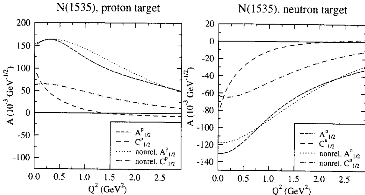
Figure 6: N(1535) electroexcitation helicity amplitudes A_{1/2}^p and A_{1/2}^n (dashed curves), and C_{1/2}^p and C_{1/2}^n (long-dashed curves). The dotted and dot-dashed curves give the corresponding nonrelativistic result for the Breit-frame transverse and C_{1/2} helicity amplitudes, respectively.
