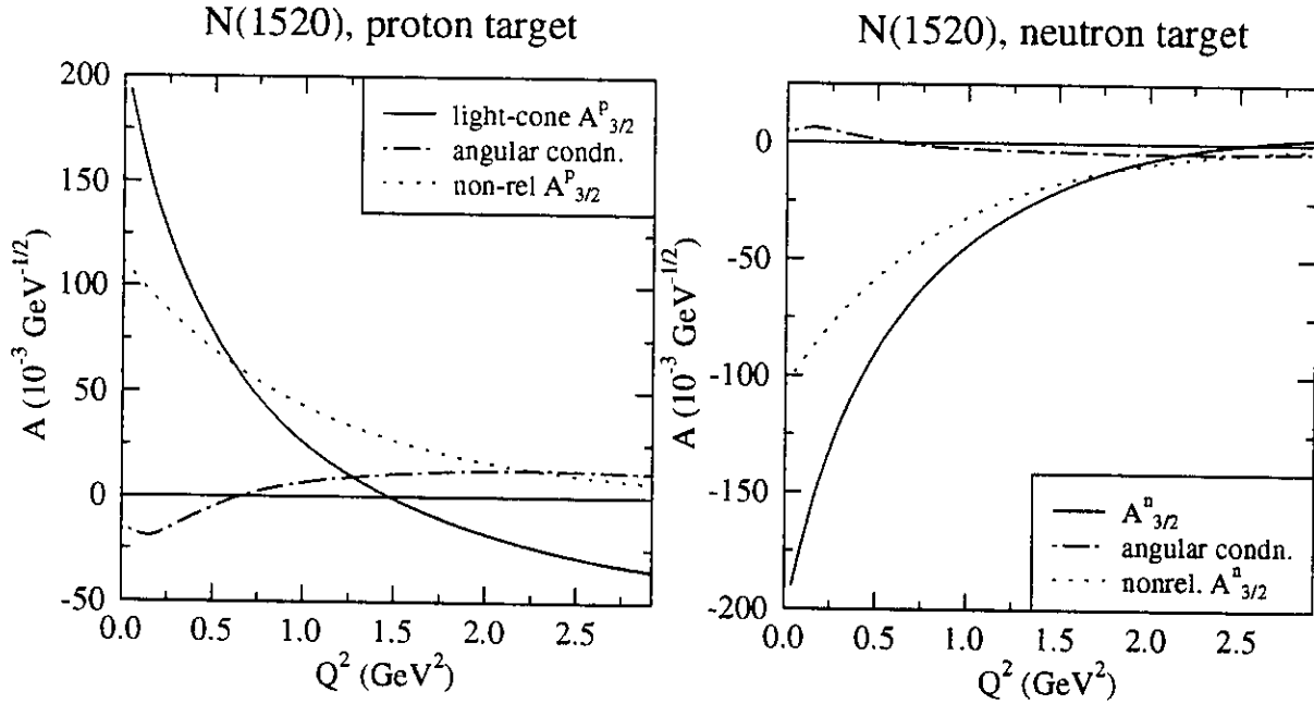
Figure 8: N(1520) electroexcitation helicity amplitudes A_{3/2}^p and A_{3/2}^n (solid curves), and the value of the rotational covariance condition (dot-dashed curve). The dotted curves give the corresponding nonrelativistic results for the Breit-frame transverse helicity amplitudes.
