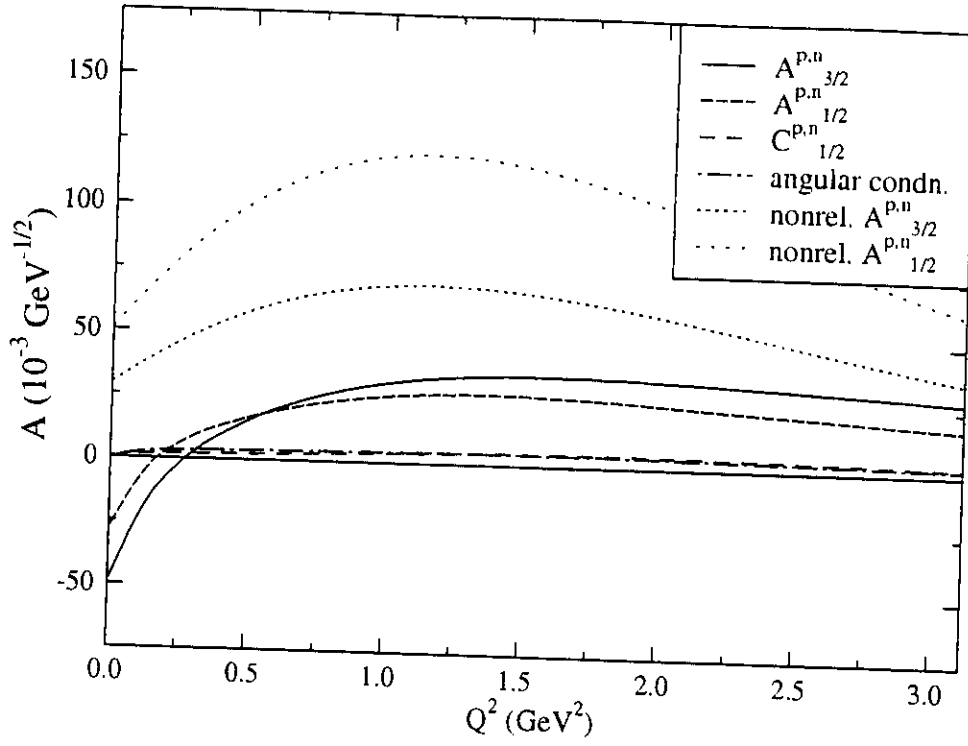
Figure 5: \Delta(1600) electroexcitation helicity amplitudes. Key as in Fig. 2 (here also the nonrelativistic amplitudes C_{1/2}^{p,n} are zero).
