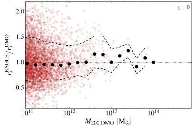
Figure 12. Ratio of NFW scale radii, r_s , in matched relaxed haloes in the DMO and EAGLE simulations. The black points are placed at the geometric mean of the ratios in each mass bin.
