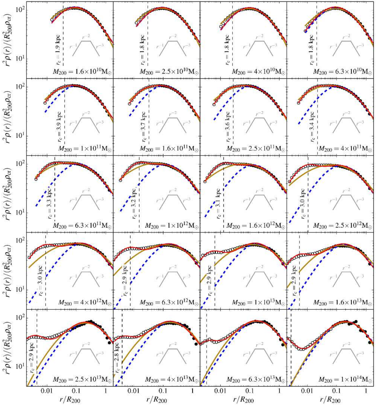
Figure 8. Stacked density profiles of the total mass normalized by the average R_{200} radius and scaled by r^2 for haloes of different masses. The filled circles are the data points used to fit an NFW profile following Neto et al. (2007), i.e. radial bins above data points below it are shown using fainter symbols. The blue dashed lines correspond to the NFW fit to the filled circles, while the brown lines correspond to an Einasto profile fit to all radial bins up to the convergence radius, r_c . The red solid line is the best-fitting profile given by equation (19), which includes an NFW contribution for the outer parts of the haloes and an additional contribution around the centre to model the baryons. The best-fitting parameters for each mass bins are given in Table 2.
