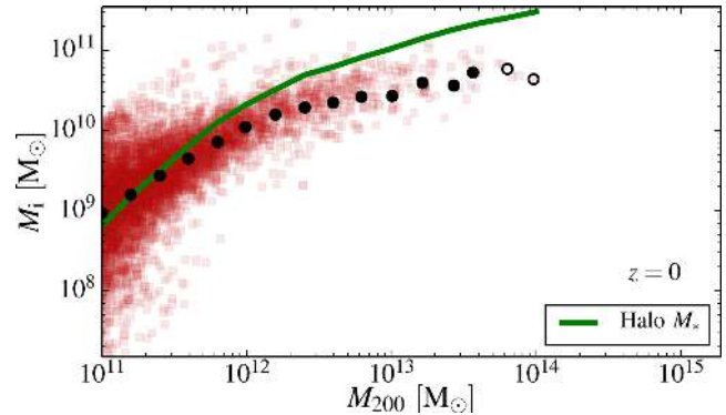
Figure 15. The mass, M_i , defined in equation (25), as a function of halo mass, M_{200} . The red squares correspond to the individual haloes and the overlaying black circles to the stacked profiles. The green solid line is the stellar mass–halo mass relation from the EAGLE simulation (Schaye et al. 2015).
