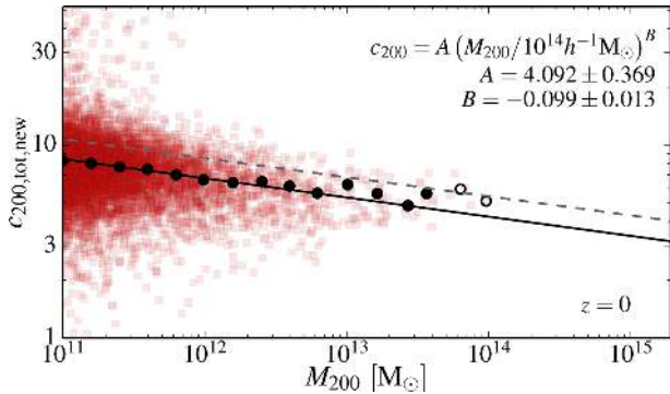
Figure 13. Halo concentration, c_{200} , as a function of mass, M_{200} , for the total matter density profiles of the EAGLE simulation using the fitting function of equation (19) and the r_s parameter to define the concentration, c_{200} = R_{200}/r_s . The colour points are for individual haloes and the black circles for the stacked profiles in each mass bin. The solid black line is the best-fitting power law (equation 23) to the solid black circles. The best-fitting values are given in the legend at the top right. The dashed line shows the best-fitting power law to the haloes extracted from the DMO simulation fitted using an NFW profile.
