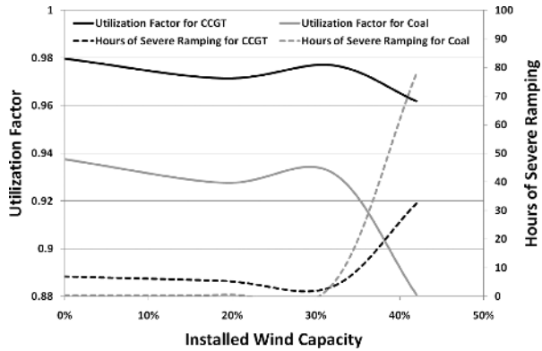
Fig. 2. Utilization factor and annual number of hours where severe ramping is performed for an average CCGT and coal unit with increasing wind penetration.
