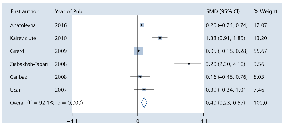
Figure 2. Forest plot of standard mean difference (SMD) for association between baseline level of interleukin-6 and occurrence of postoperative atrial fibrillation; CI — confidence interval; Pub — publication
