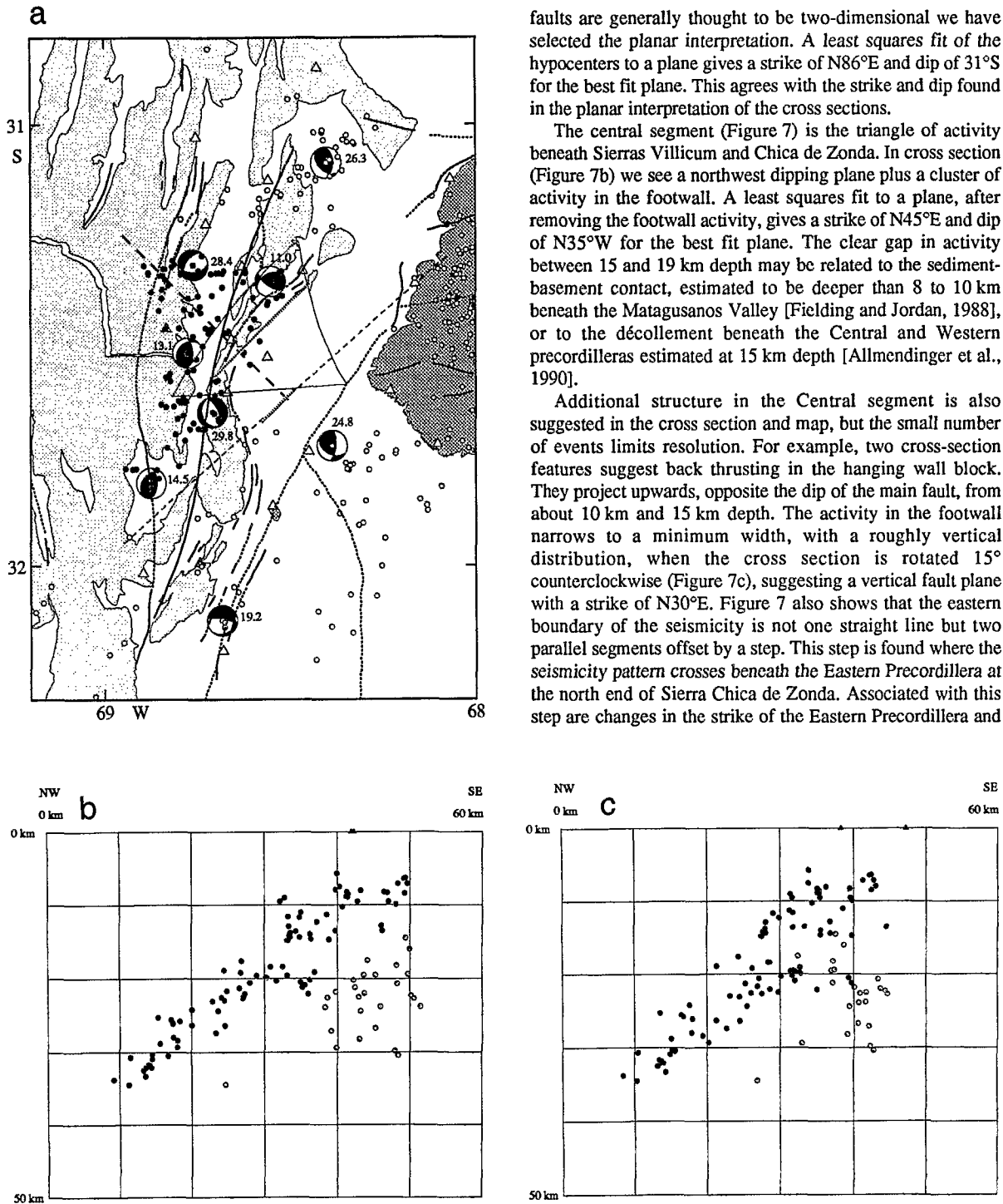
Fig. 7. (a) Map and (b,c) cross sections of locations for central segment (solid circles). A cross section (b) striking N45°W has the steepest dip (35°NW) and a good planar distribution indicating a fault plane striking N45°E and dipping NW. The surface intercept of the proposed fault (long southwest to northeast dashed line), and the cross section strike (northwest to southeast dashed line through center segment) are shown on the map. The projection of the ends of the LANDSAT lineament near La Laja are shown in the cross section by the small triangles. Map and earthquake symbols are as in Figure 6. A tightening of the activity in the footwall block into a less well-defined vertical plane is seen when the cross section is rotated to a strike of N60°W (c) indicating a vertical plane that strikes N30°E.
