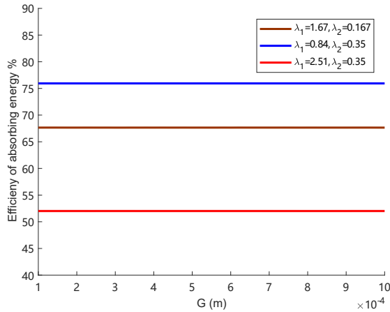
Fig. 13. Maximum energy dissipation ratio that a best tuned K system for certain excitation G can achieve under the different damping parameters conditions
