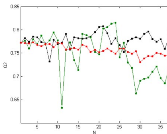
Figure F20. Comparative leave- N -out crossvalidation plot for the MLR model on data set 1. Black - single LNO, red - multiple LNO (10 times), and green - single LNO using the original (not randomized) data set.
