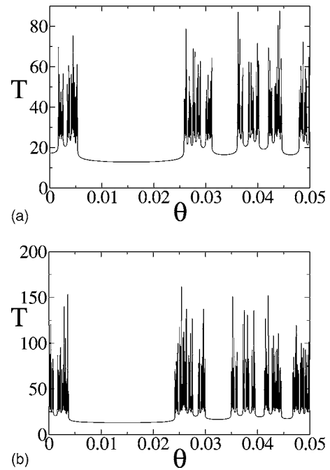
FIG. 5. Typical delay-time function for the conservative (a) and the weakly dissipative (b) Hénon-Heiles system with chaotic scattering ( E=0.19 , \alpha=10^{-4} , and \beta=10^{-4} ).
