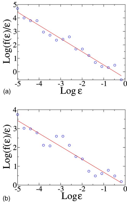
FIG. 6. For E=0.19 in the Hénon-Heiles system so that there is chaotic scattering, algebraic scaling of f(\epsilon)/\epsilon with \epsilon . The absolute value of the slope from a linear fit gives a good estimate for the fractal dimension of the set of singularities in the delay-time function. We obtain D=0.97\pm 0.01 for the conservative case and D=0.71\pm 0.02 for the weakly dissipative case.
