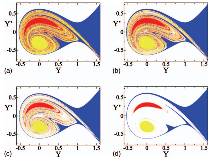
FIG. 9. (Color) (a)–(d) Basins of scattering destinations and of the fixed-point attractor at the center of the scattering region for E = 0.19 and for \mu = 5 \times 10^{-4}, 10^{-3}, 10^{-2} , and 10^{-1} , respectively.
