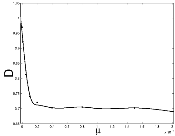
FIG. 7. The uncertainty dimension D versus the dissipation parameter \mu = \alpha = \beta . The rapid decrease in D for \mu \geq 0 is characteristic of a cusp.
