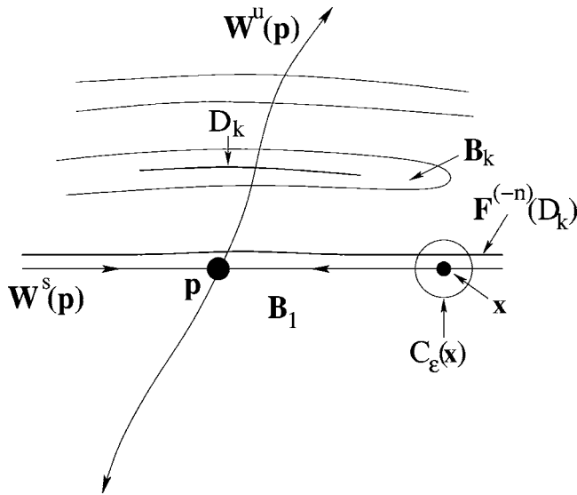
FIG. 10. Schematic illustration of the Kennedy-Yorke theorem establishing the Wada property. See the text for details.
