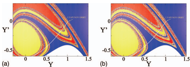
FIG. 11. (Color) For E=0.25 in the Hénon-Heiles system, a segment of the unstable manifold of one of the three Lyapunov orbits, an unstable periodic orbit accessible to at least one basin. That the segment intersects all four basins suggests the Wada property of the basins, (a) in the Hamiltonian case, (b) in the dissipative case with \alpha=10^{-4} , and \beta=10^{-4} .
