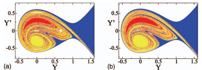
FIG. 8. (Color) For E=0.19 in the Hénon-Heiles system, (a) the basins of scattering particles in the conservative case. In this case, there are three destinations, and initial conditions going to the destinations are distinguished by three colors and the white regions inside the plotted structure denote the KAM islands. (b) The basin structure in the presence of a small amount of dissipation ( \alpha=10^{-4} and \beta=10^{-4} ). Due to the dissipation, an additional destination arises: the fixed point at the center of the scattering region. Four colors are then needed to distinguish the initial conditions. See the text for simulation details.
