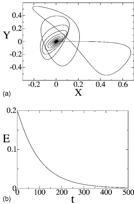
FIG. 4. (a) In the presence of dissipation ( \alpha=0.1 and \beta=0.1 ), a particle permanently trapped in the scattering region. The corresponding trajectory approaches the fixed-point attractor in the phase space. (b) Exponential decay to zero of the particle energy when it approaches the attractor.
