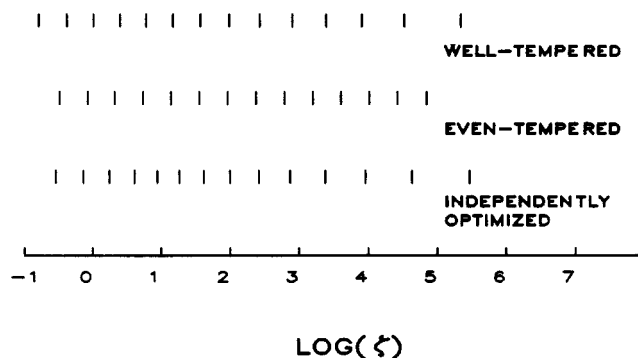
Figure 1. The distribution of s-symmetry gaussian exponents in three energy-optimized (14s,9p) neon atom basis sets.
